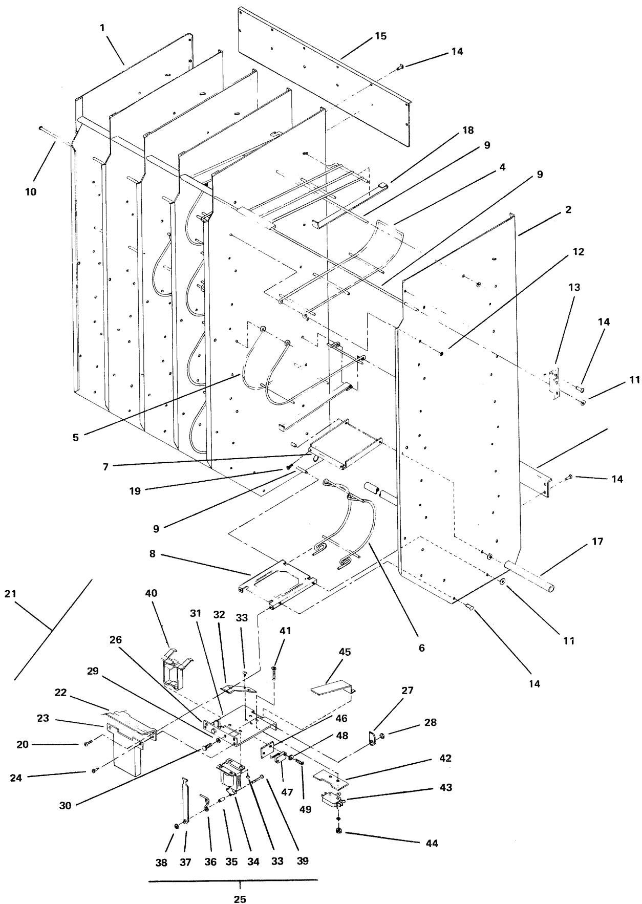
Figure 4 CAN RACK ASSEMBLY 19
