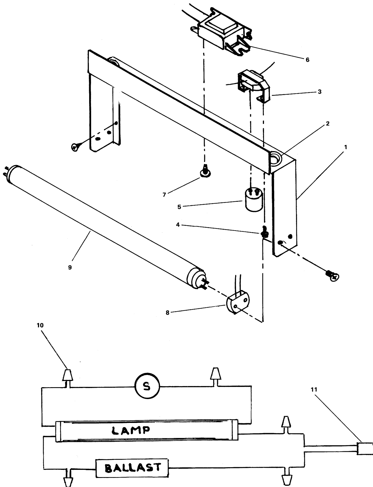
FIGURE 9 LIGHT ASSEMBLY
