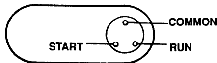
SCHEMATIC #1
